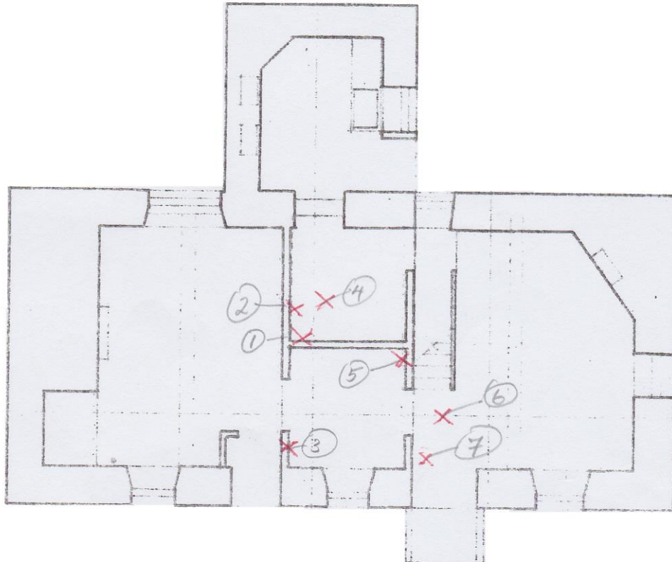
Figure 1: Ground floor plan of Hendy Groes, showing the approximate locations of the samples taken.
