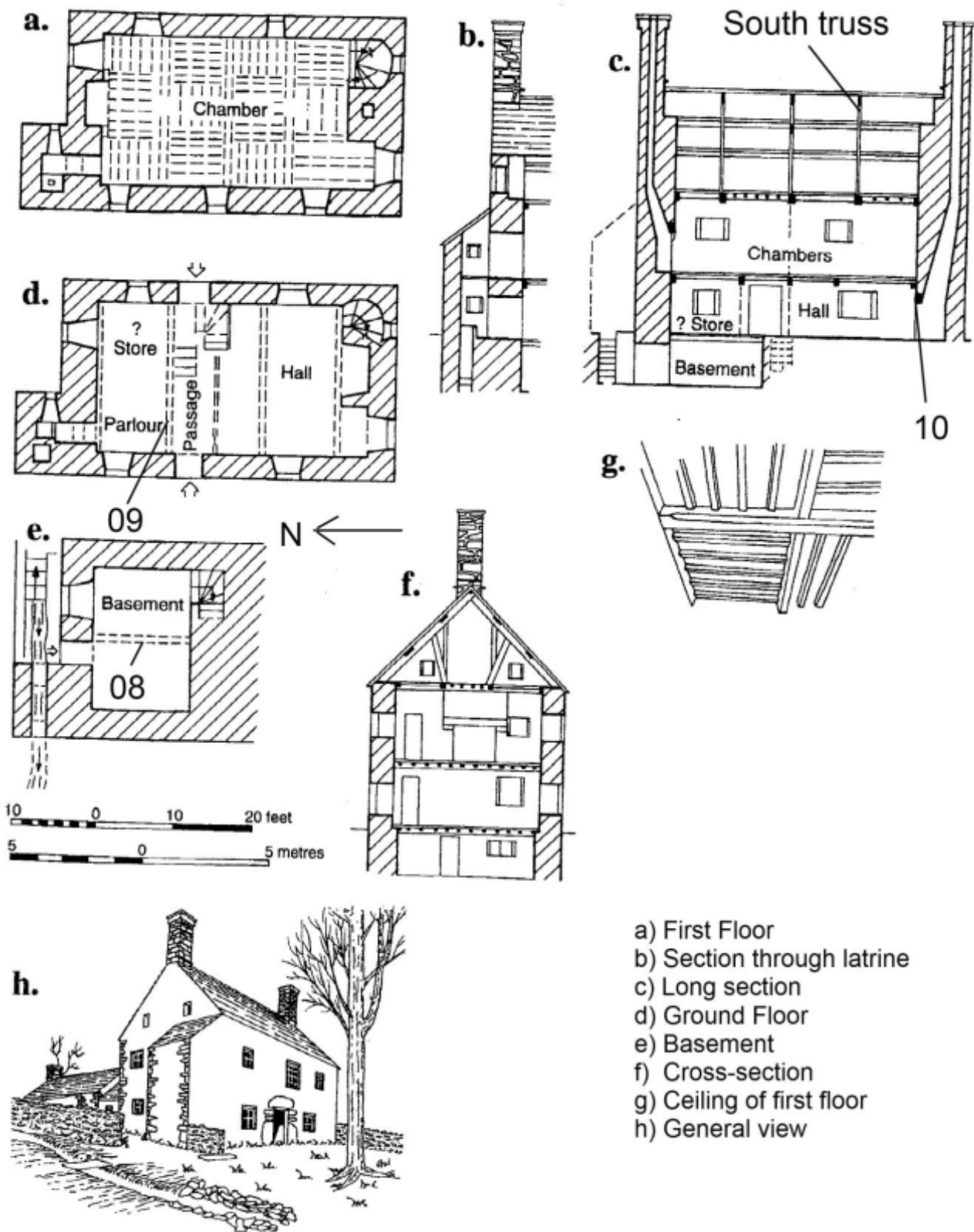
Figure 1: Drawings of the building adapted from Smith 2001 (Fig 10.44) to show some of the timbers sampled for dendrochronology
